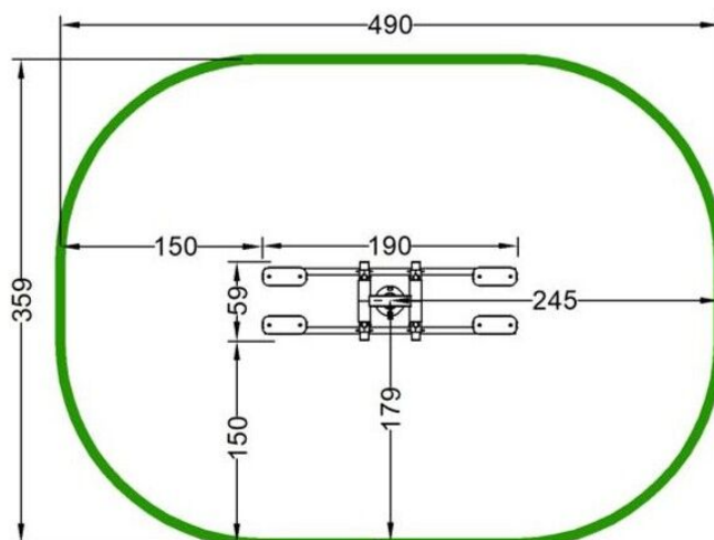
Device and impact area dimensions
