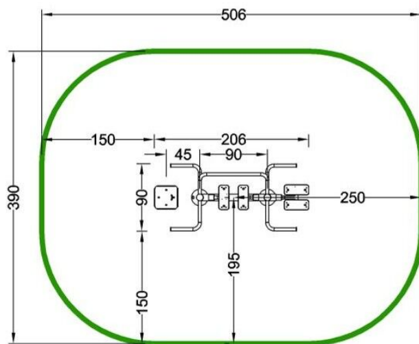
Device and impact area dimensions
