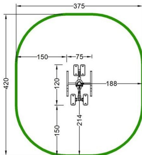
Device and impact area dimensions
