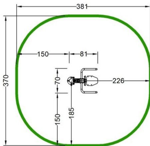
Device and impact area dimensions
