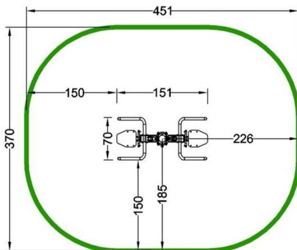
Device and impact area dimensions
