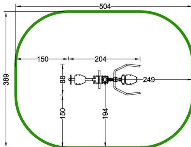
Device and impact area dimensions
