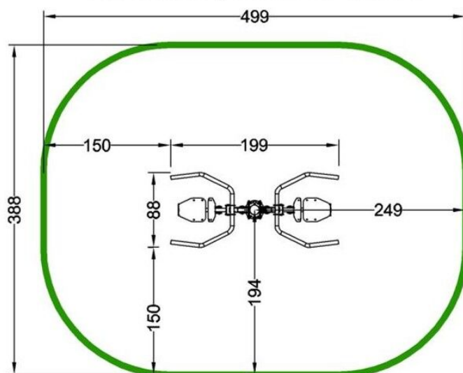
Device and impact area dimensions
