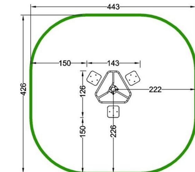
Device and impact area dimensions
