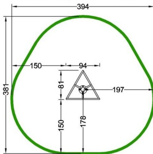
Device and impact area dimensions
