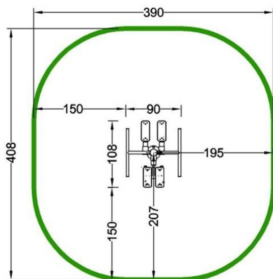
Device and impact area dimensions
