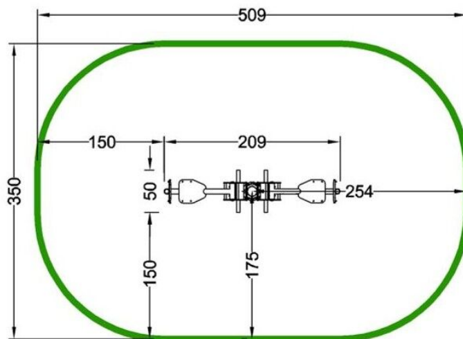
Device and impact area dimensions
