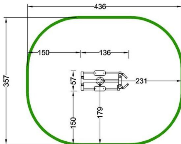
Device and impact area dimensions
