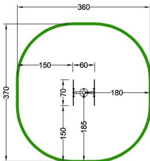
Device and impact area dimensions
