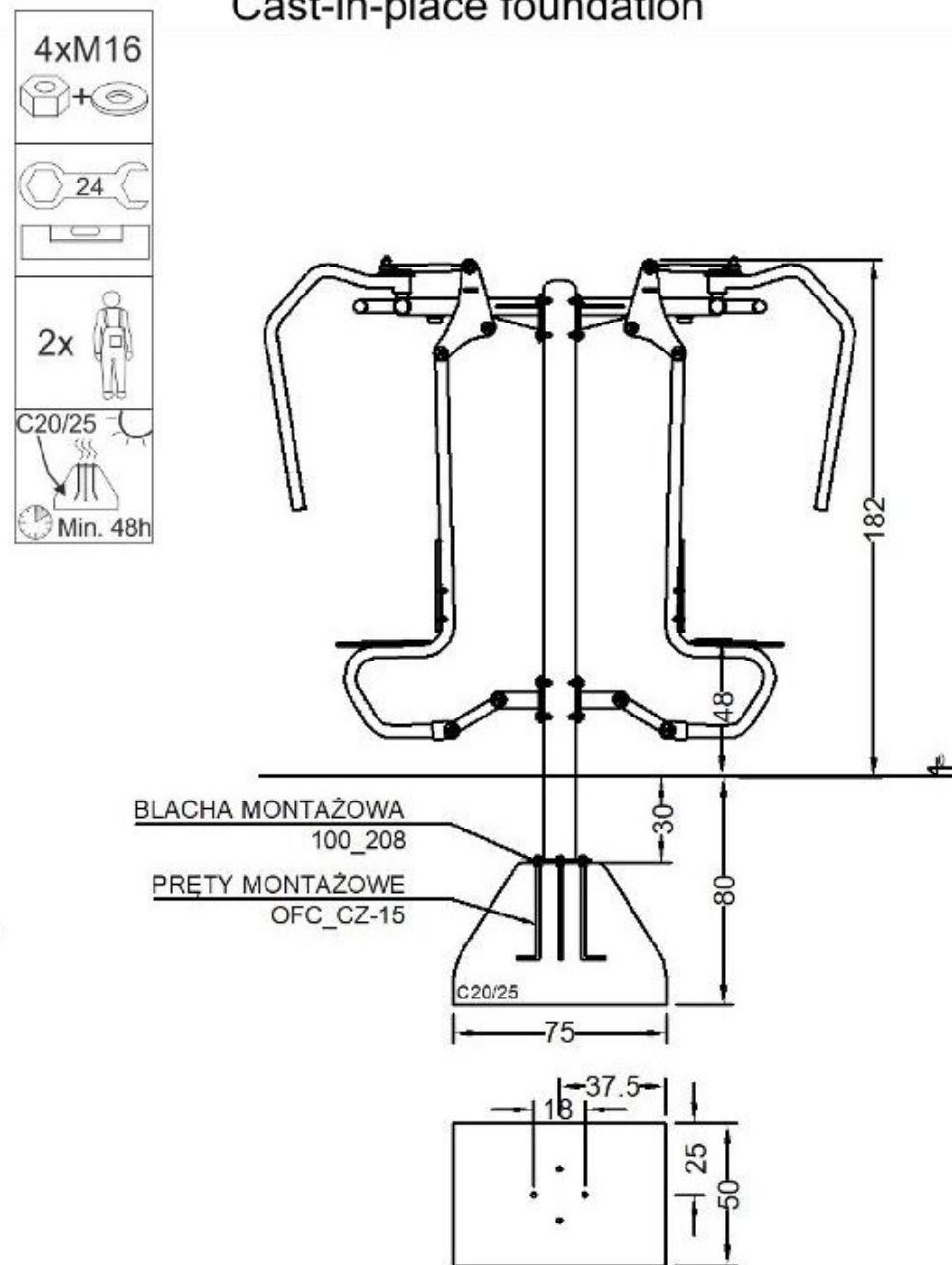
Cast-in-place foundation
