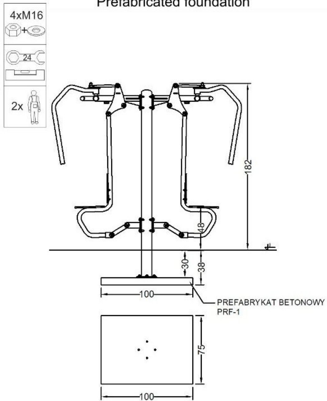
Prefabricated foundation
