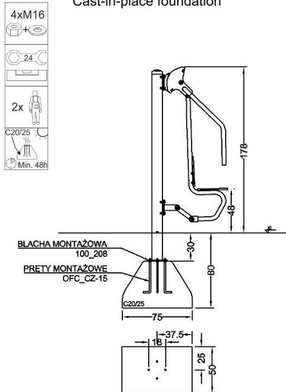
Cast-in-place foundation
