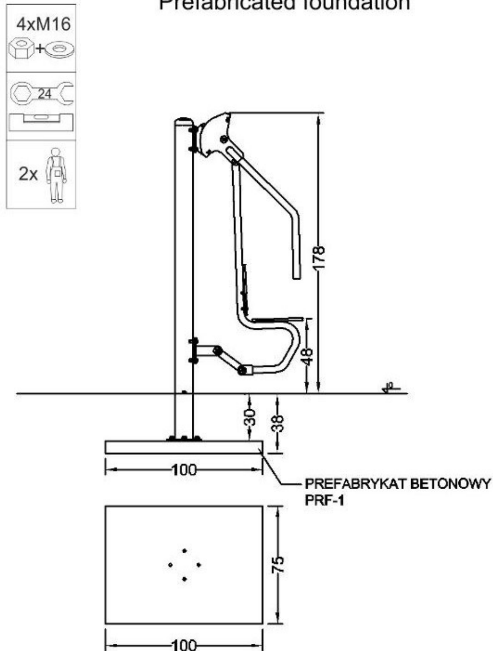
Prefabricated foundation
