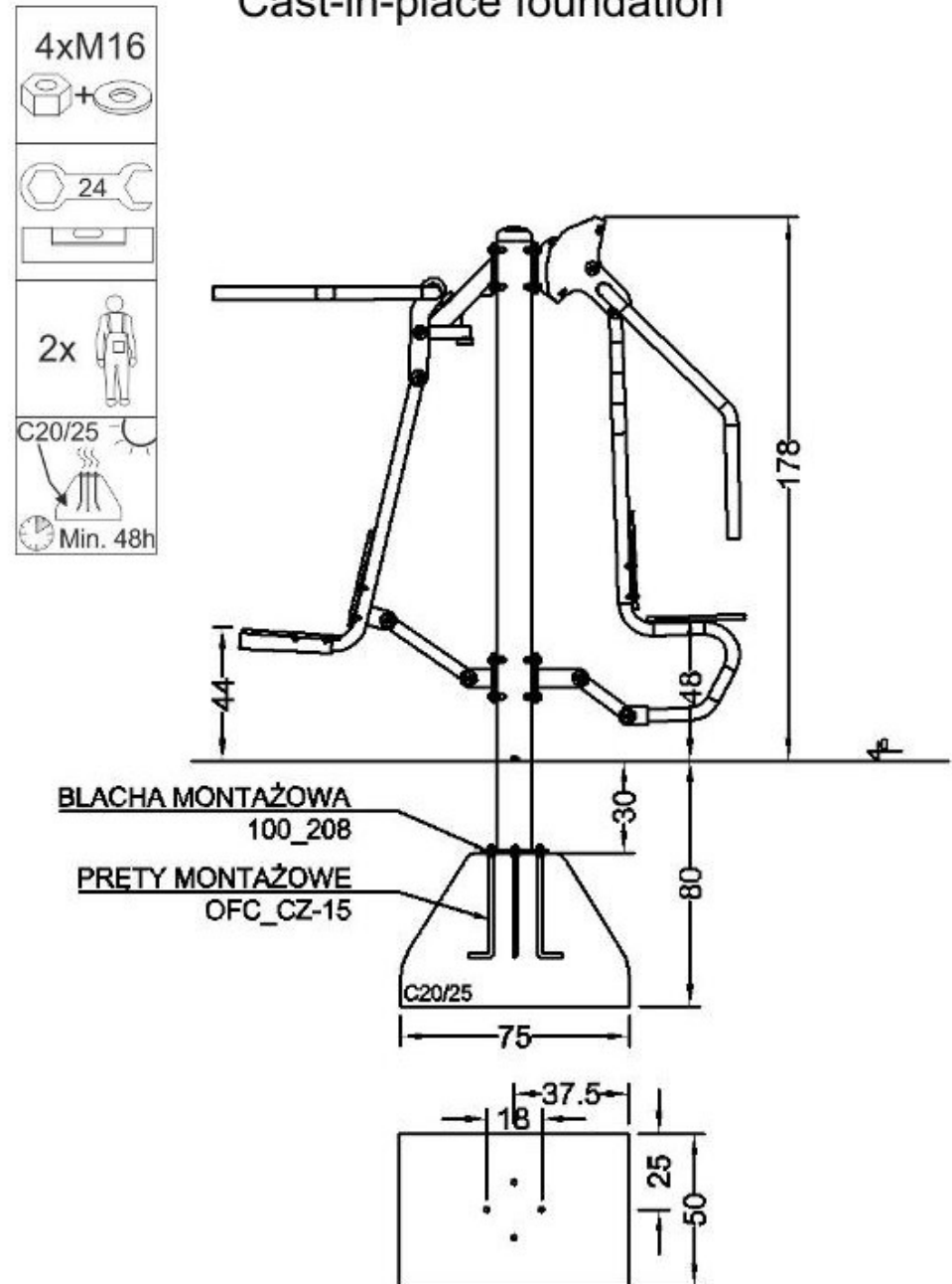
Cast-in-place foundation
