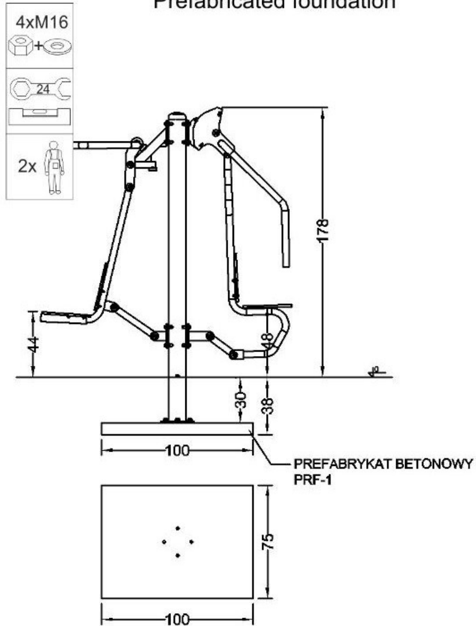
Prefabricated foundation
