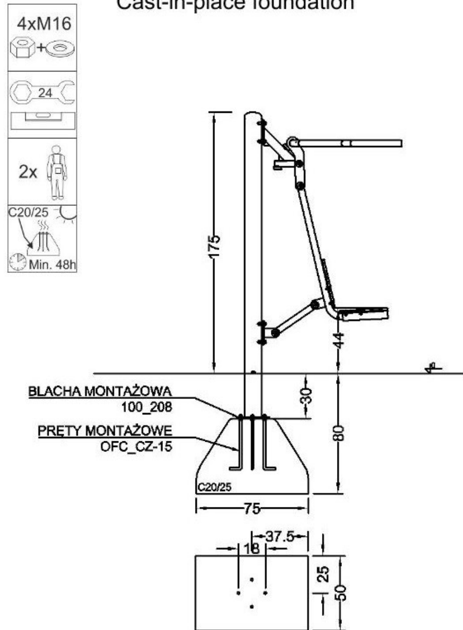
Cast-in-place foundation
