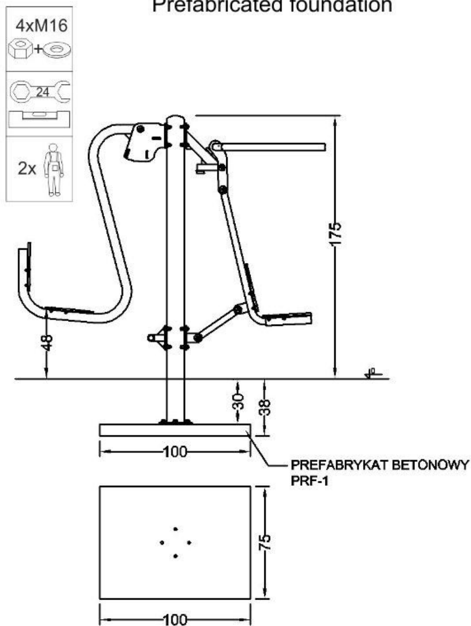
Prefabricated foundation
