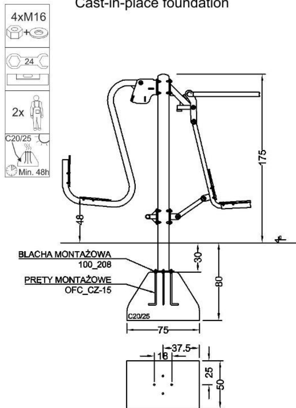
Cast-in-place foundation
