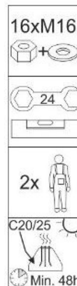
Cast-in-place foundation
