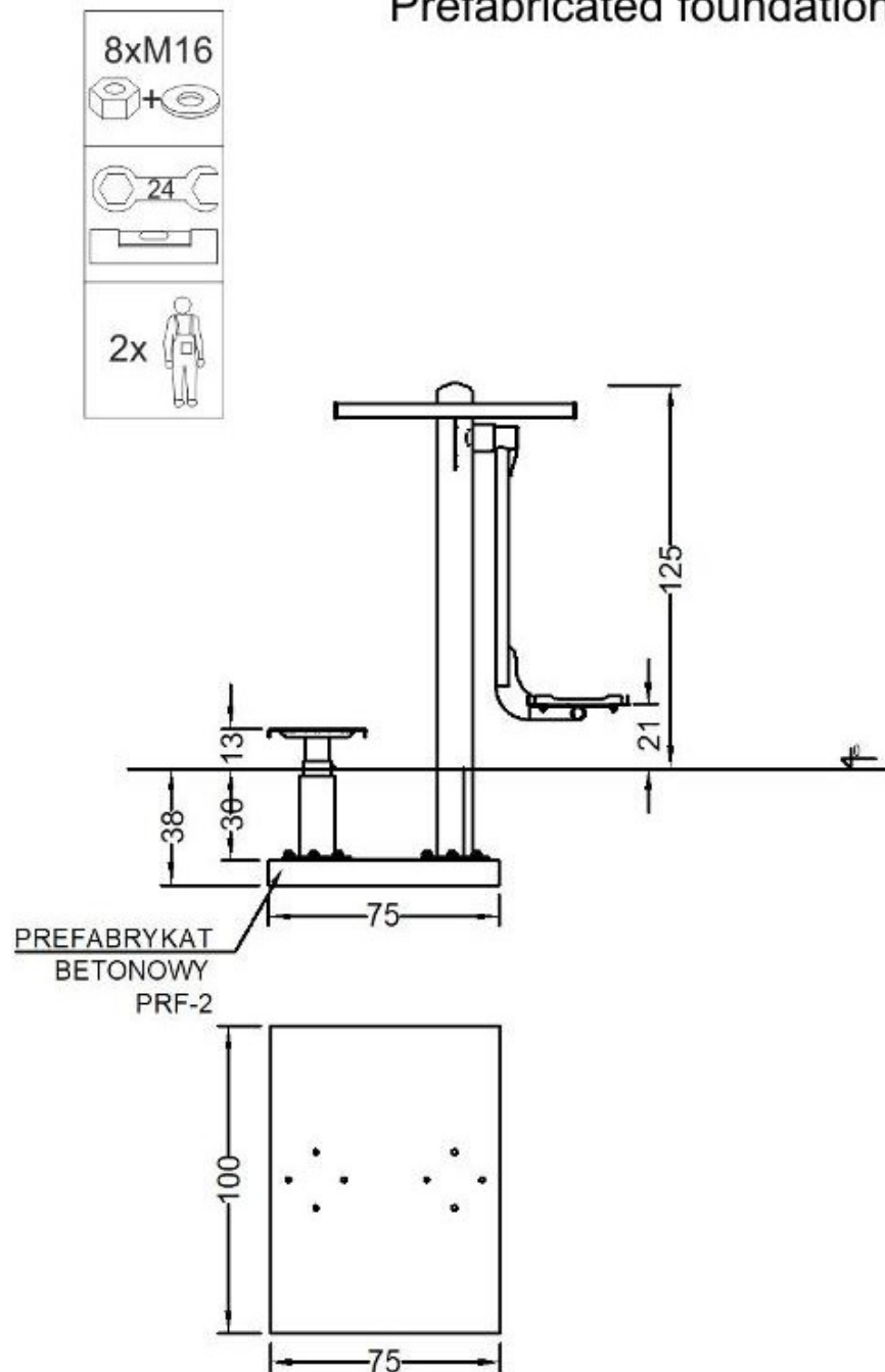
Prefabricated foundation
