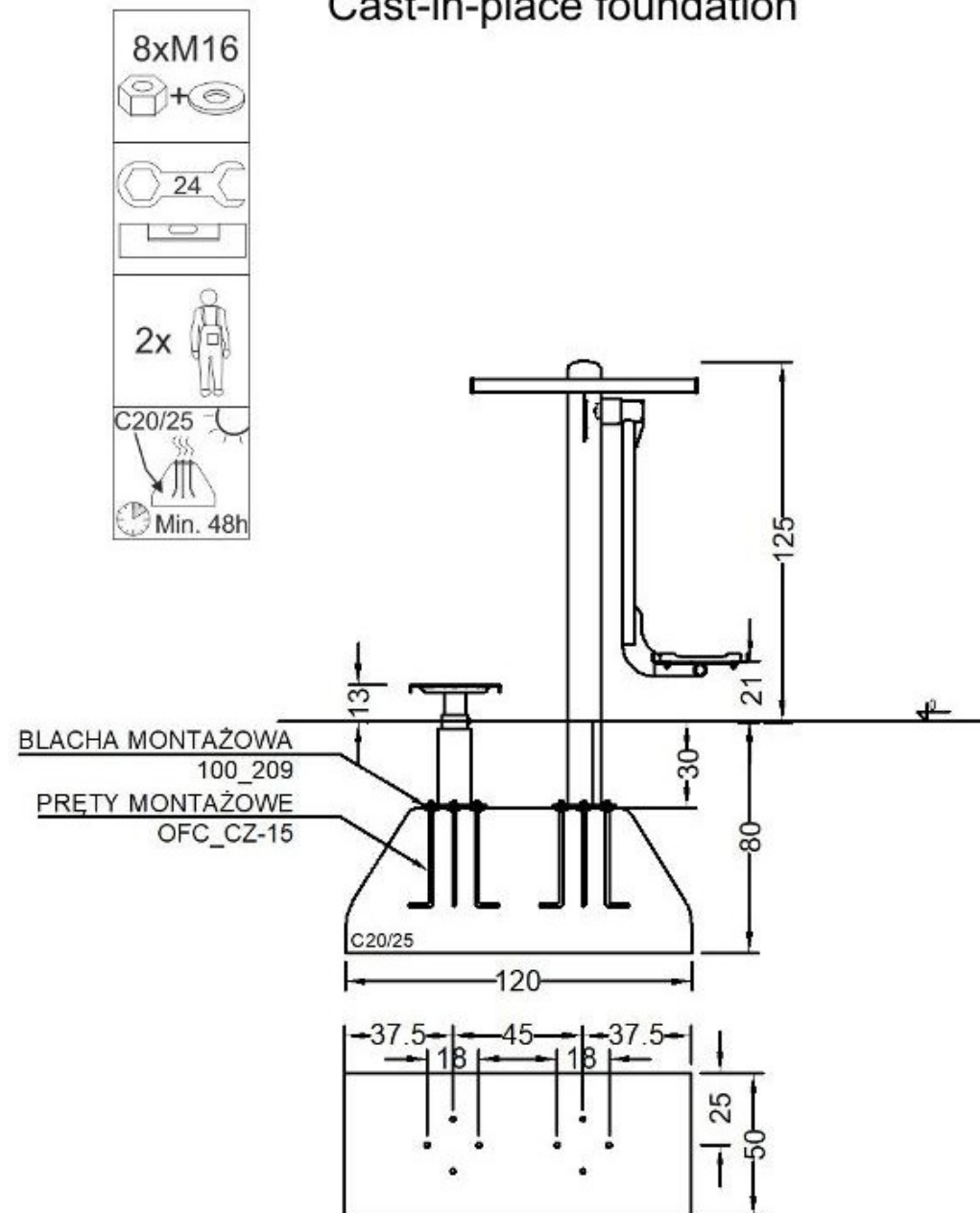
Cast-in-place foundation
