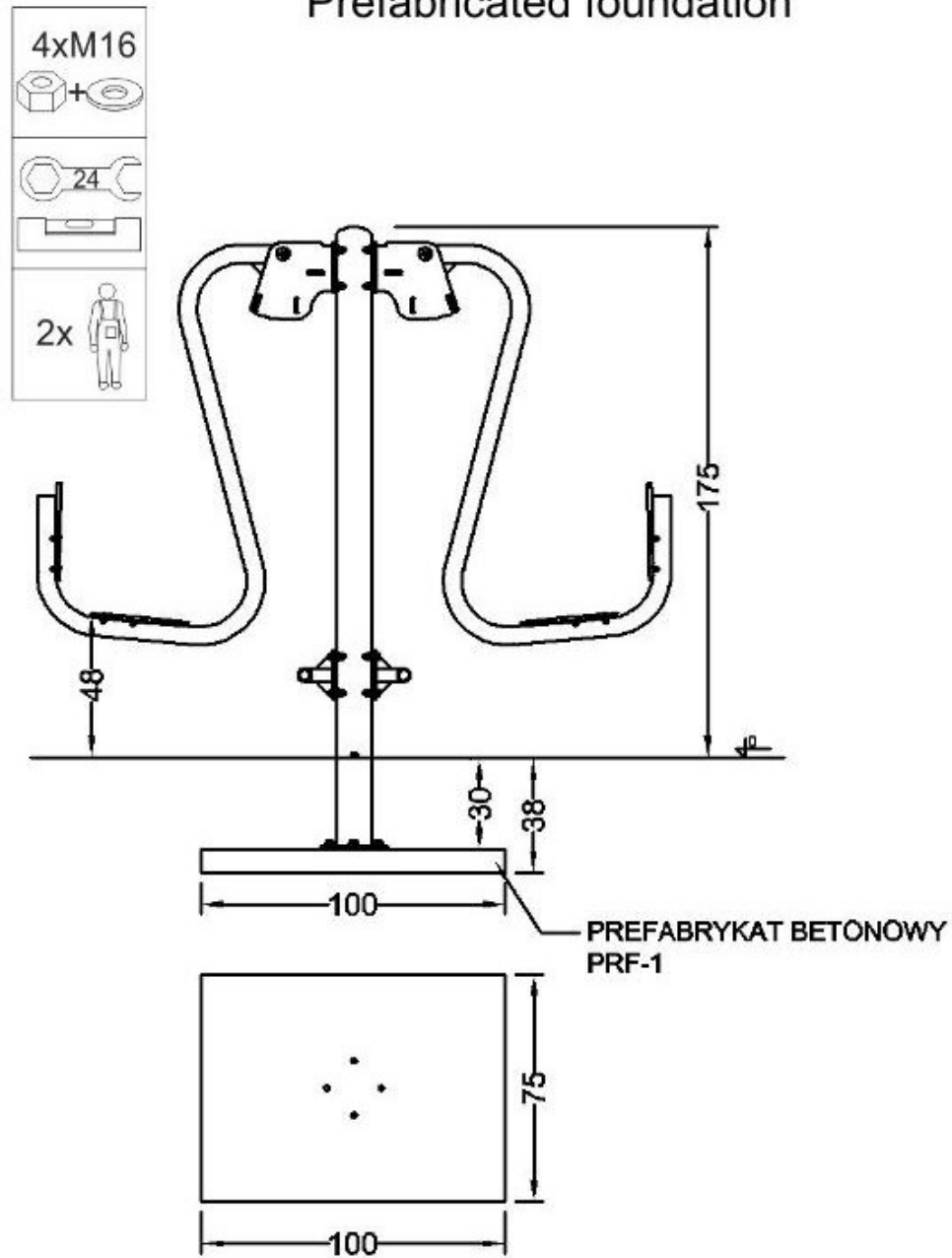
Prefabricated foundation
