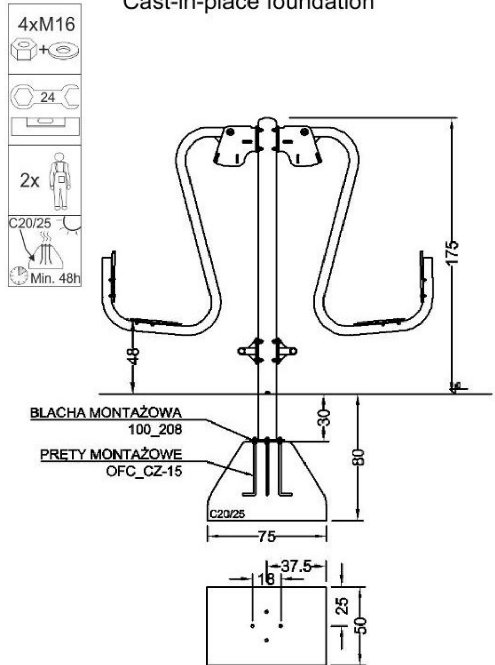
Cast-in-place foundation
