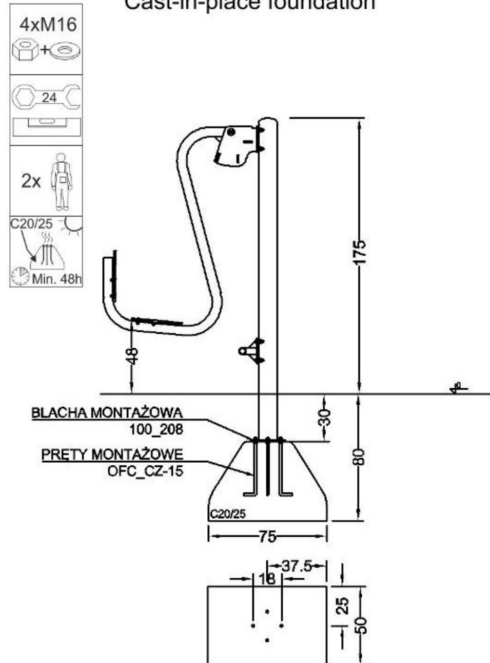
Cast-in-place foundation
