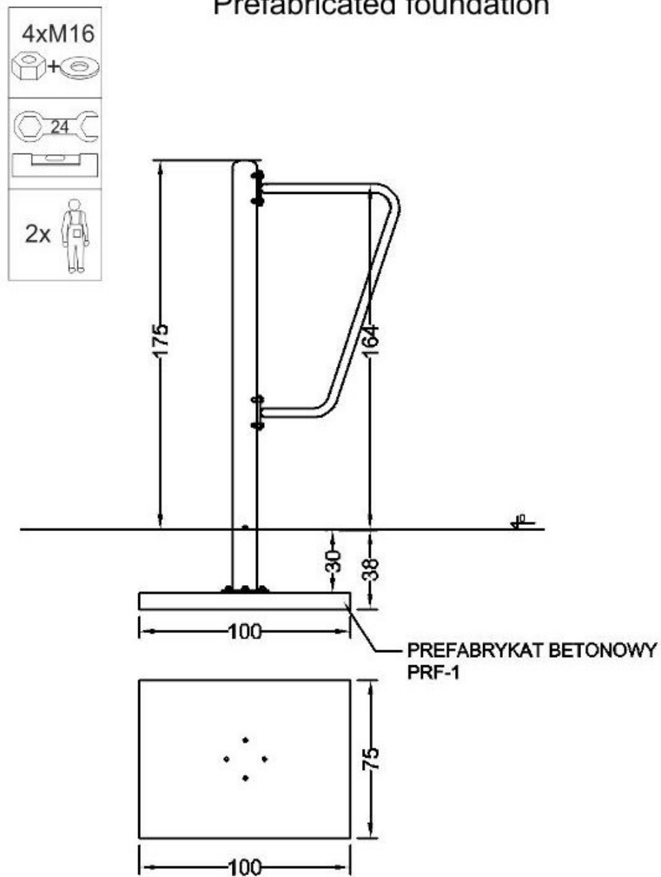
Prefabricated foundation
