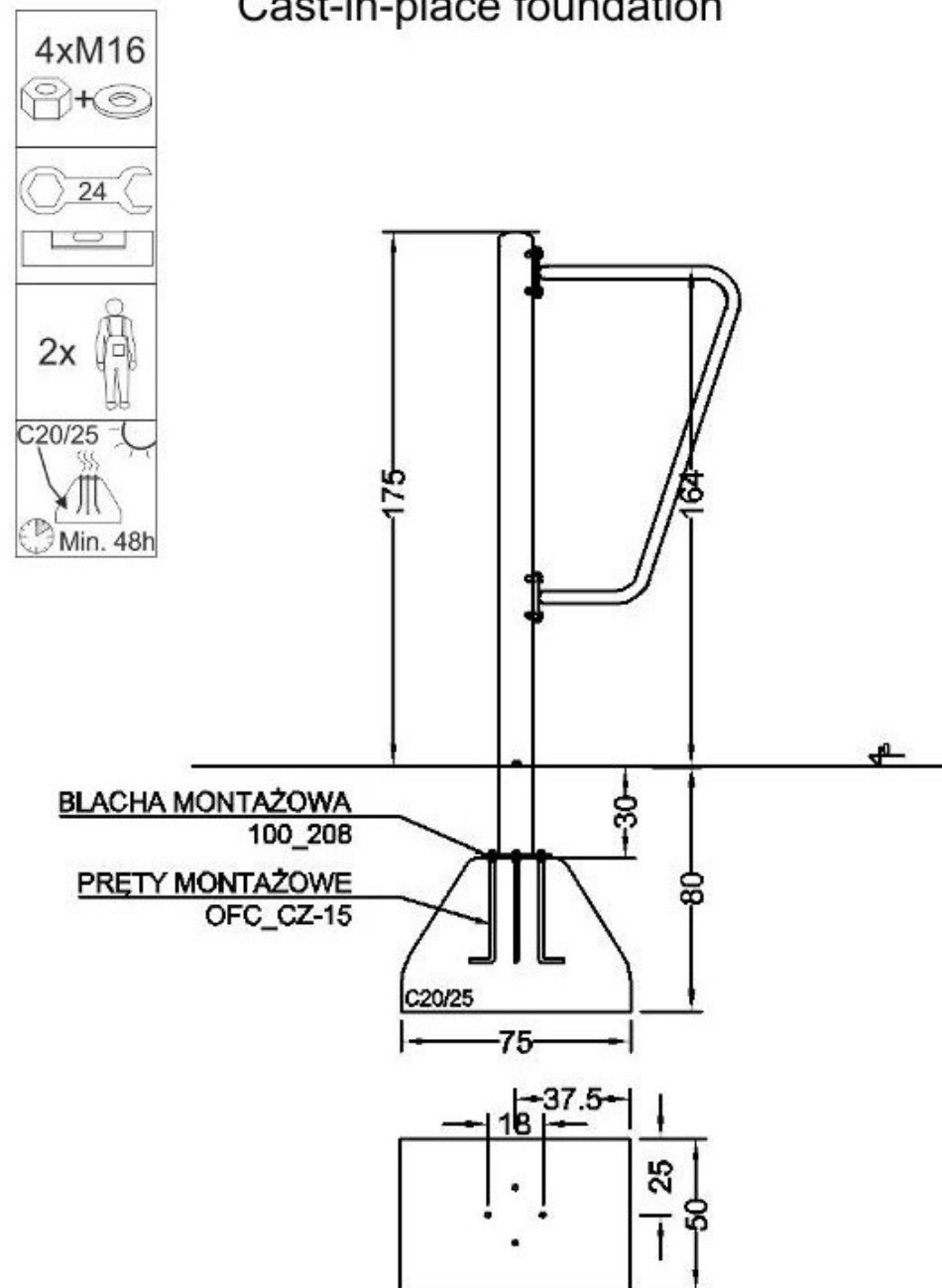
Cast-in-place foundation
