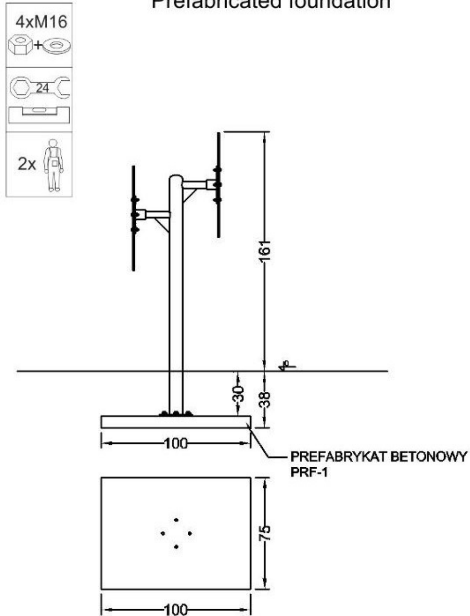
Prefabricated foundation
