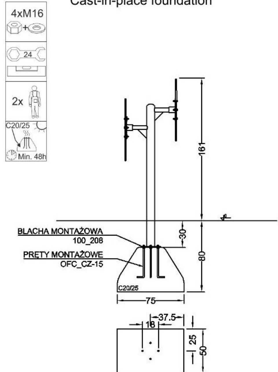
Cast-in-place foundation
