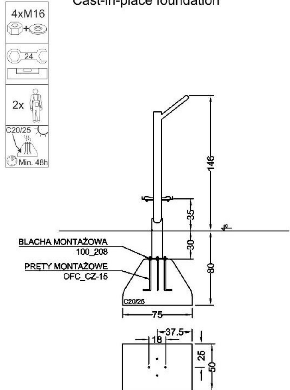
Cast-in-place foundation
